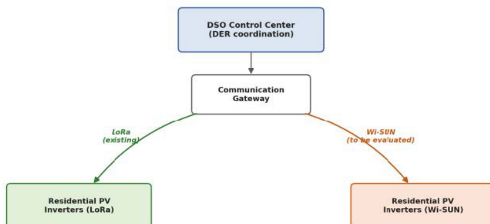
Target communication architecture between the DSO control center and residential PV inverters
