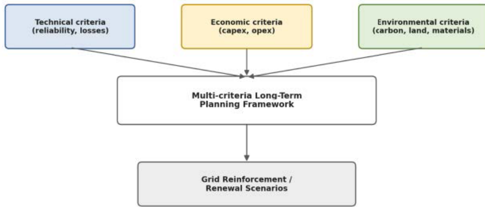
Multi-criteria long-term distribution grid planning framework
